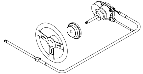
NFB™ 4.2 Dual Cable System (Steering Wheel not included.)
